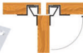
RH- 1609 SSF BRASS W - TYPE HINGES
